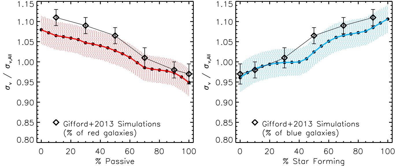
Figure 10. The velocity dispersions estimated from resampling the ensemble cluster data while controlling for the fraction of passive and star-forming galaxies included in each resampling. In both panels we plot our results while over-plotting values (open diamonds) from a similar analysis of simulated galaxy clusters from Gifford et al. (2013), where the simulated galaxy clusters are populated with galaxies using a variety of different halo-tracking and semi-analytic prescriptions. The simulated work uses a binary red vs. blue galaxy classification, and so we show two panels here where the only difference between the two is in how we treat post-starburst galaxies in our dataset—i.e., whether they are grouped in with passive or star-forming galaxies. Left : In this panel we vary the fraction of passive galaxies used in the resampling, using the combined post-starburst+star-forming samples to replace passive galaxies as the passive galaxy fraction is decreased. Right : In this panel we vary the fraction of star-forming galaxies used in the resampling, using the combined passive+post-starburst samples to replace star-forming galaxies as the star-forming galaxy fraction is decreased.
