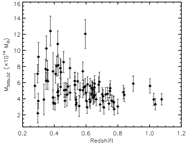
Figure 1. The redshift distribution and SZ-derived masses of the galaxy clusters used in this work, all SZ-selected. Masses are taken from Bleem et al. (2015) and Hasselfield et al. (2013).
